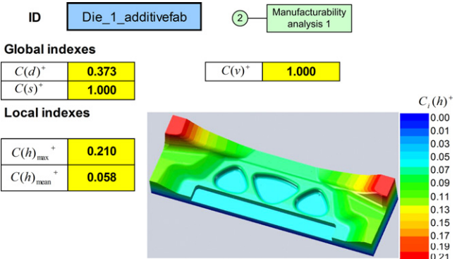
Fig. 14. Manufacturability analysis for additive manufacturing.
