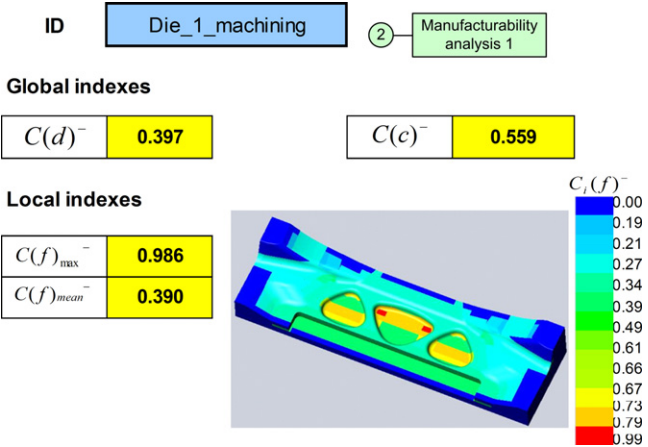
Fig. 13. Manufacturability analysis for machining.
